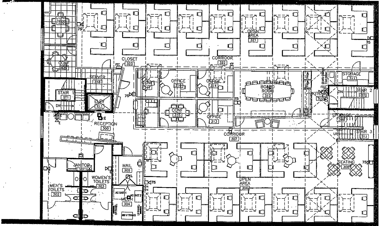
THIRD FLOOR PLAN 1/8" = 1'-0"
