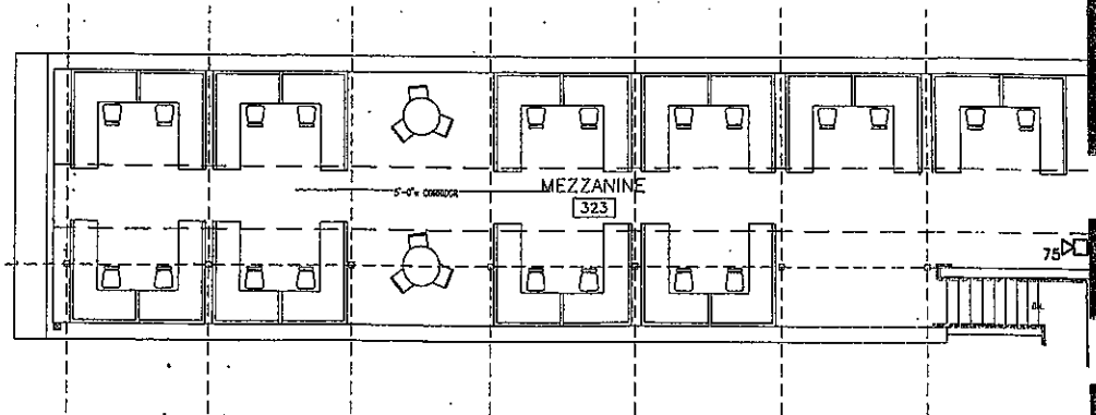
THIRD FLOOR MEZZANINE LEVEL 1/8" = 1'-0"
